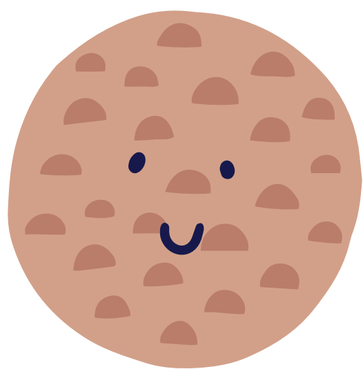
MERCURY
